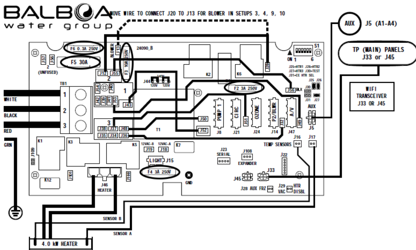
“Typical Board Layout”
